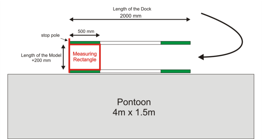
Figure 3. Sketch of the dock and the measuring rectangle. Assumed arrival from right side. If the arrival direction is from the left measuring rectangle on the right side is used.
