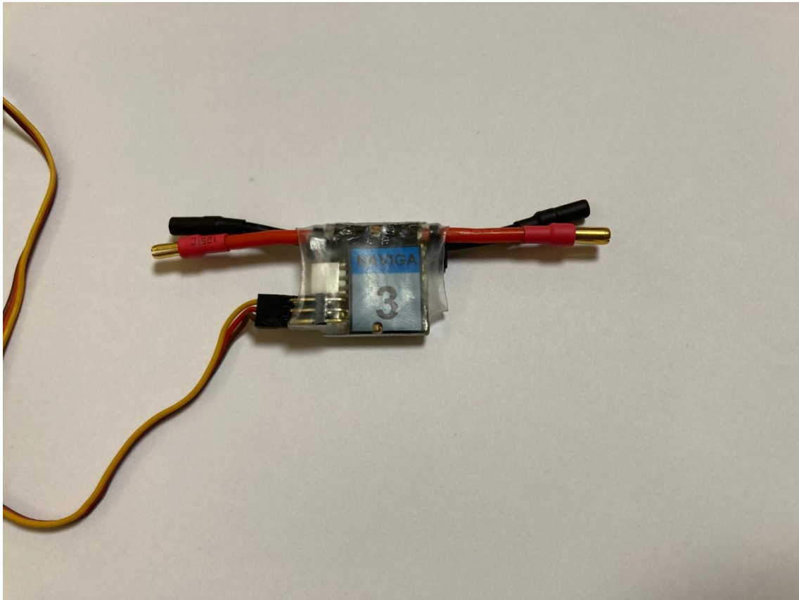
eLim mini, connectors according Naviga suggestion. - No adapter needed.
