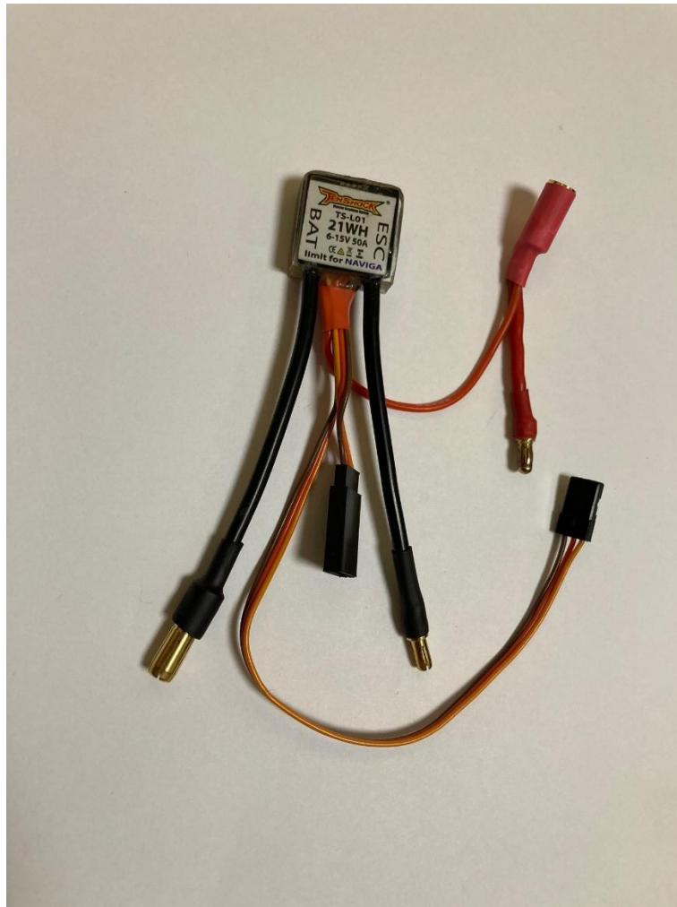
Tenshock 21Wh custom connectors – Adapter must be provided.
