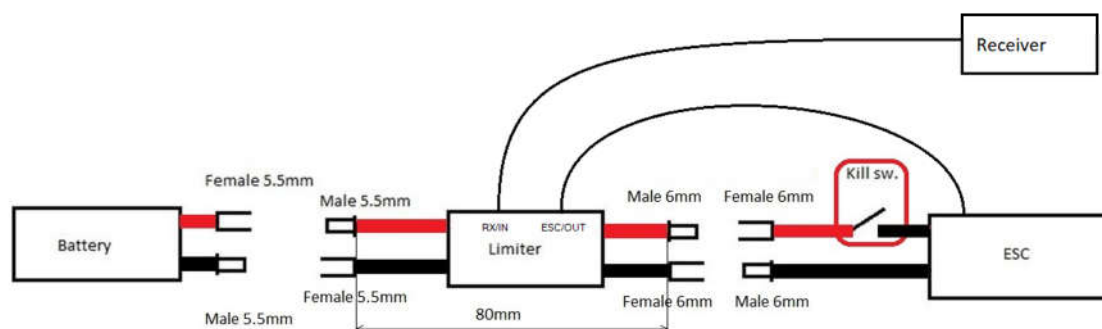
Connection diagram for Naviga provided energy limiters
